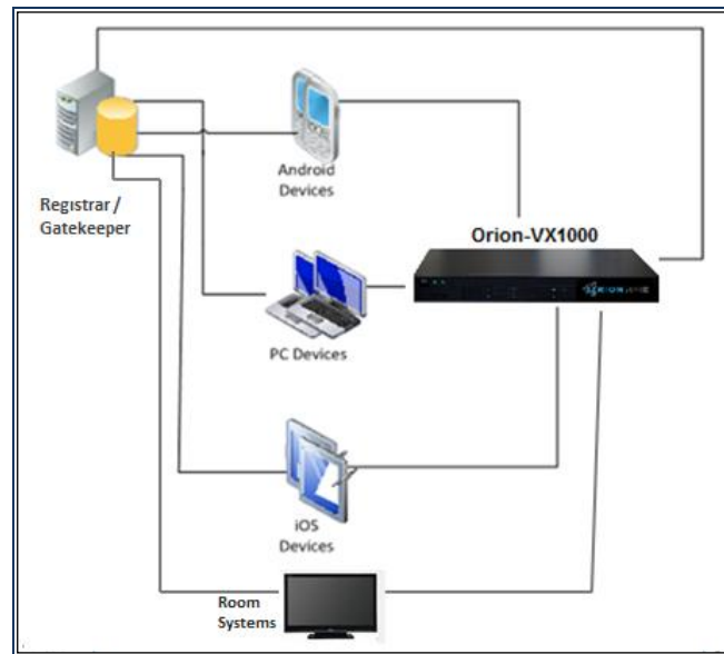
Figure 1: Orion-VX1000/VX2000/1286 Architecture
