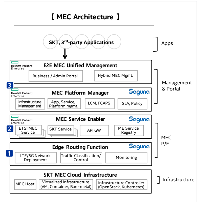
Figure 1. SK Telecom's 5G-based MEC platform architecture
