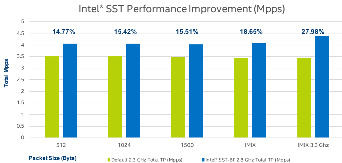
Figure 7. Layer 3 packet forwarding performance-millions of packets per second (Mpps)
