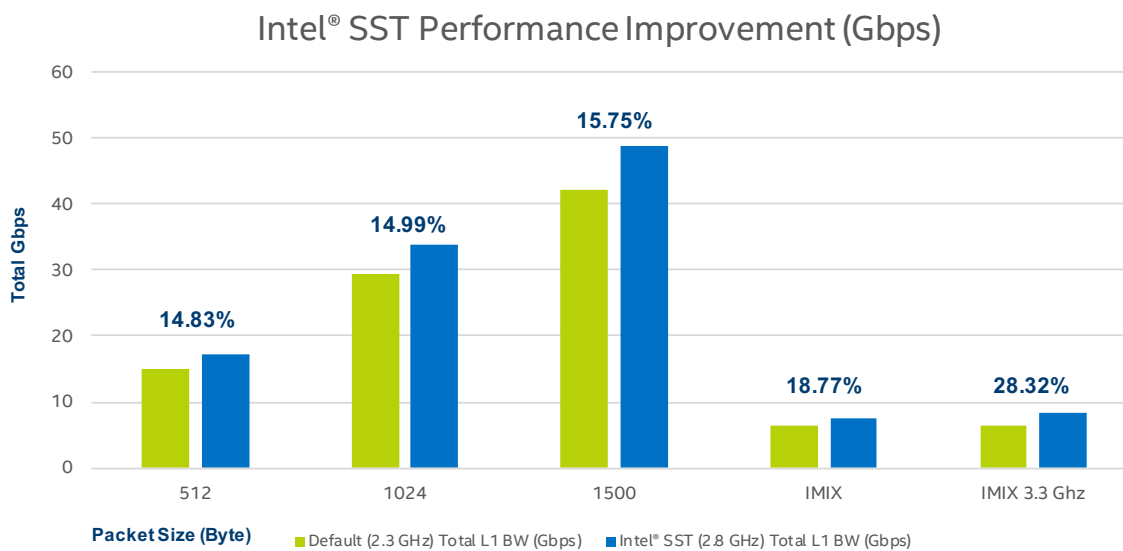
Figure 8. Layer 3 packet forwarding performance-Gbps
