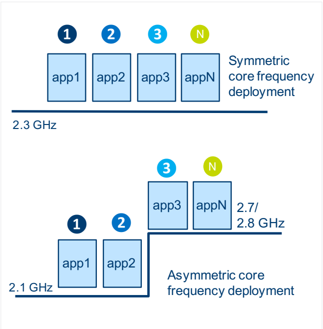
Figure 2. Intel® SST-BF
