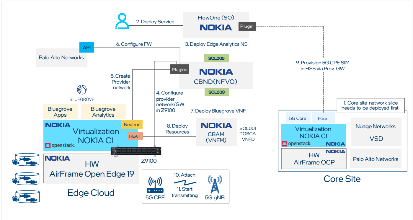
Figure 5. Service orchestration for Edge cloud and 5G CPE provisioning.
